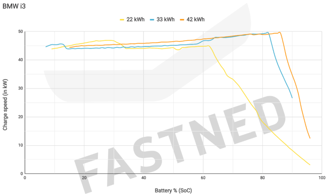
Figure 11.64: Actual charging profile of BMW i3 as a function of vehicle's SoC.
