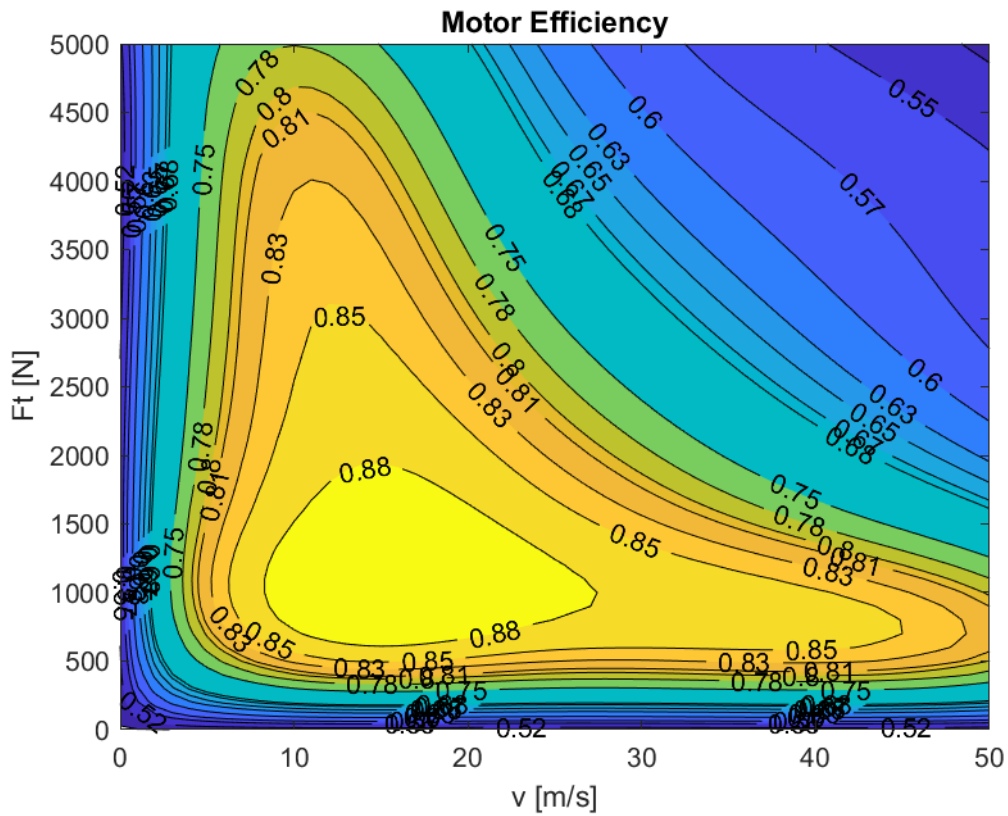
Figure 11.74: Generated 2D EV efficiency map.
