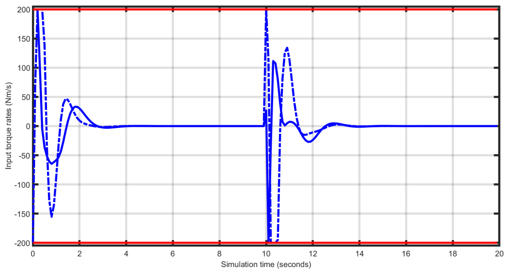
Figure 11.51: Manipulator's torque rates.
