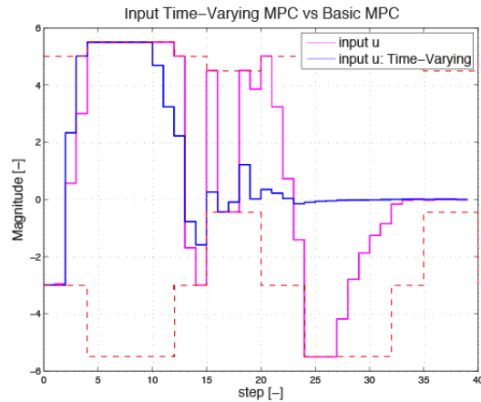
Figure 11.4: Input Time-varying MPC vs. basic MPC
