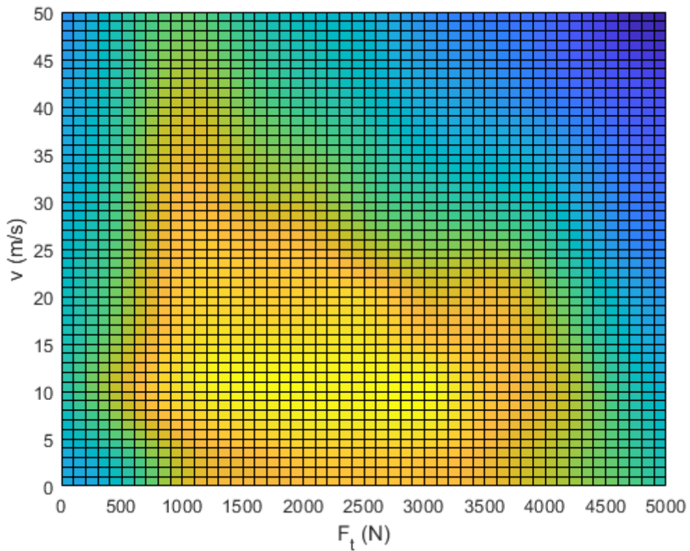
Figure 11.63: Generated 2D EV efficiency map. Note that we are using a simplified 1D efficiency map \eta(F_t) taken for v = 15 m/s in this example.
